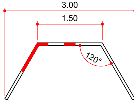
SECTION A
